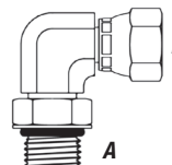
SAE M to JIC F Swivel 90° Elbow
